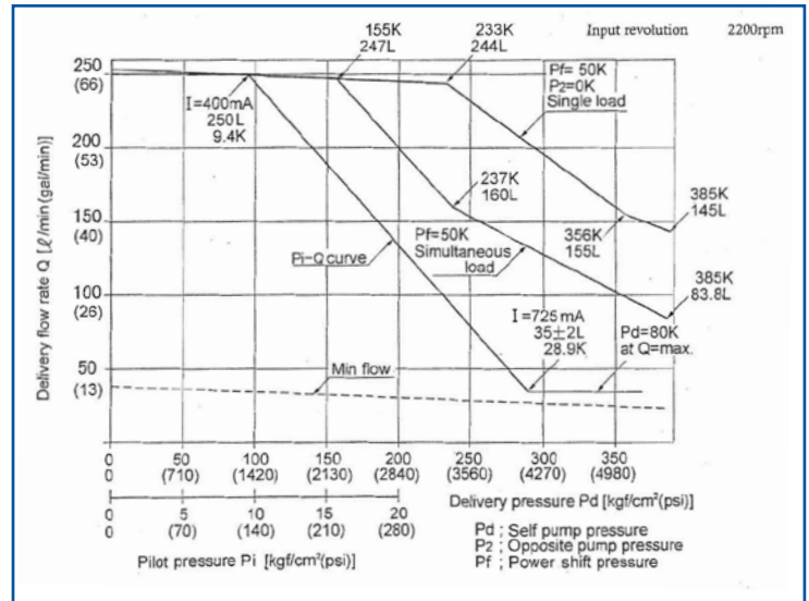
Pump HP Curve
